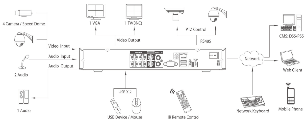
DVR3104 System Connection
